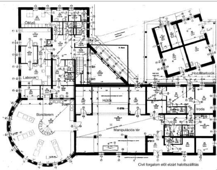
4.50. Morgue of Károlyi S. Hospital, Pathological Dept., Újpest, (1996) Architect: SCHRAMMEL, Z.
