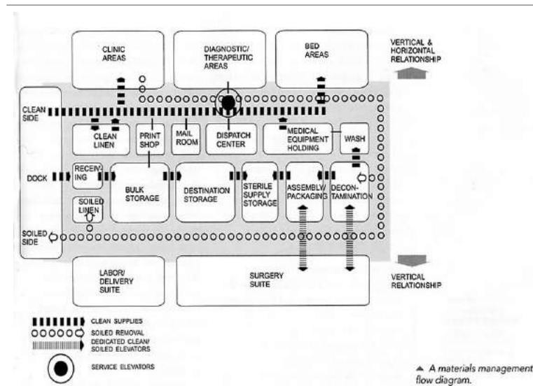
4.54. Material management flow diagram to the Central Sterilization Unit
