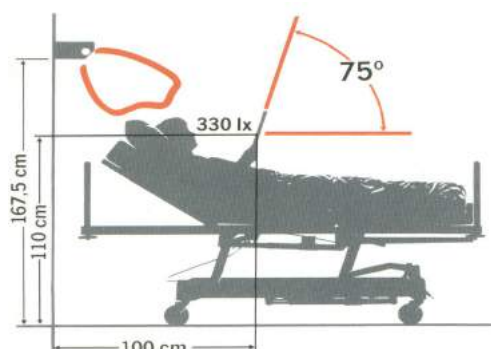
4.15. Space requirement around the bed 4.16. Down: optimal illumination (Trilux)
