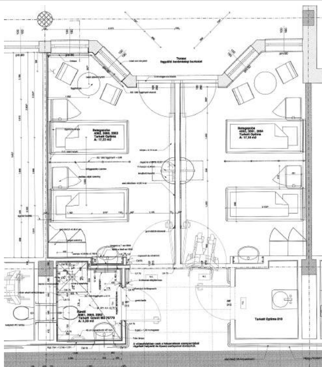
4.14. Two-bed-wards with bathroom opened from entrance bay, Szt. Imre Hospital Budapest, (2001) Arch.: SCHRAMEL Z.
