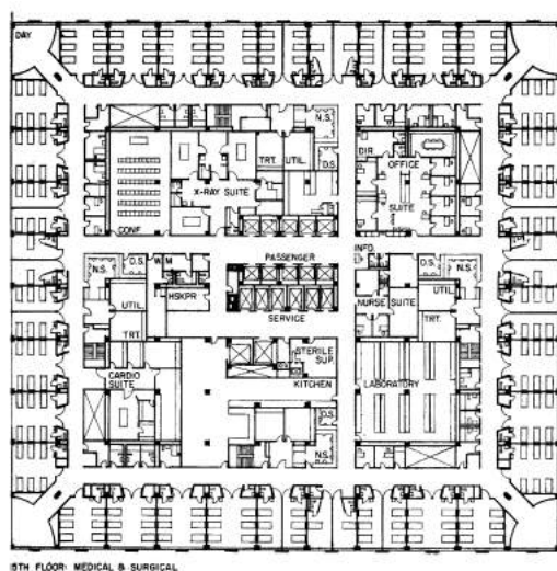
4.05. Typical hotel floor plan of an American high block hospital
