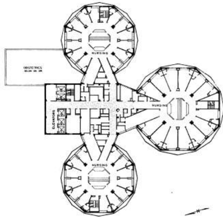
4.03. Compact circular plan, Scott and White Memorial Hospital, Texas (1964.)
