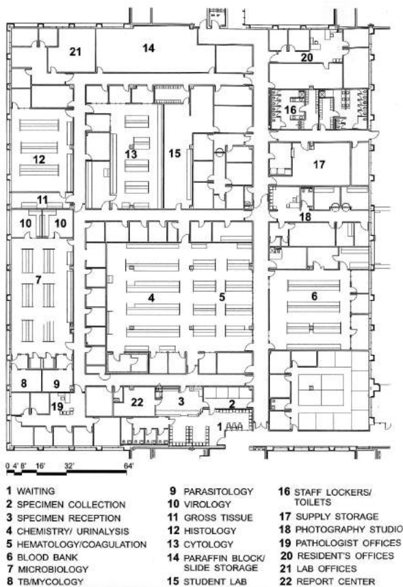
4.28. Plan of clinical laboratory, Brooke Army Medical Center, San Antonio, Texas
