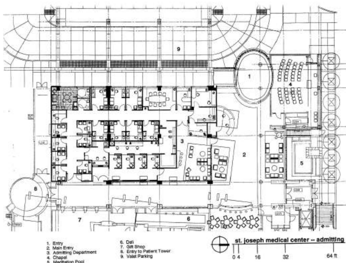
4.48. Admitting Department, St Joseph Med. Center, Tacoma USA (1993) Designer: BUFFALO Design, Inc.
