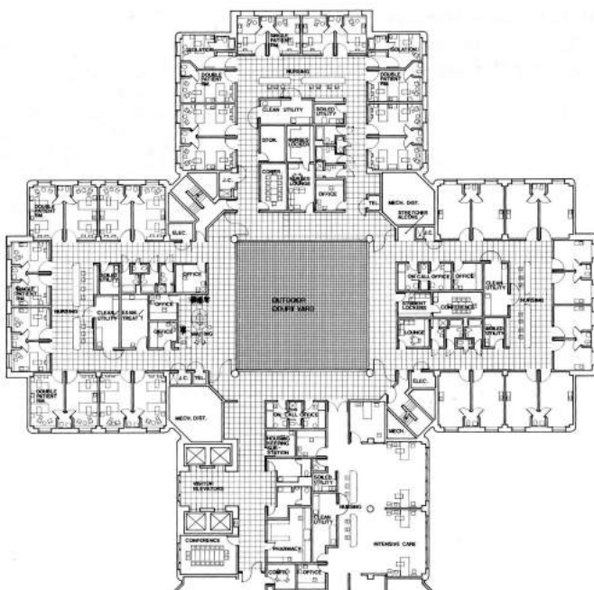
4.01. Department with 3 nursing units + intensive unit, Detroit Receiving Hospital, USA (1979)
