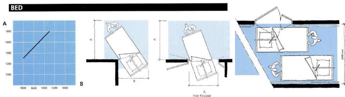
4.19. Free passage measurements for moving with beds (Arjo Guide Book)
