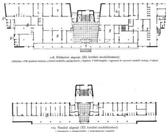
4.44. Polyclinic, Budapest. XI. Fehérvári út (1949) Ground and general floor plan Designer: SZENDRŐI J.
