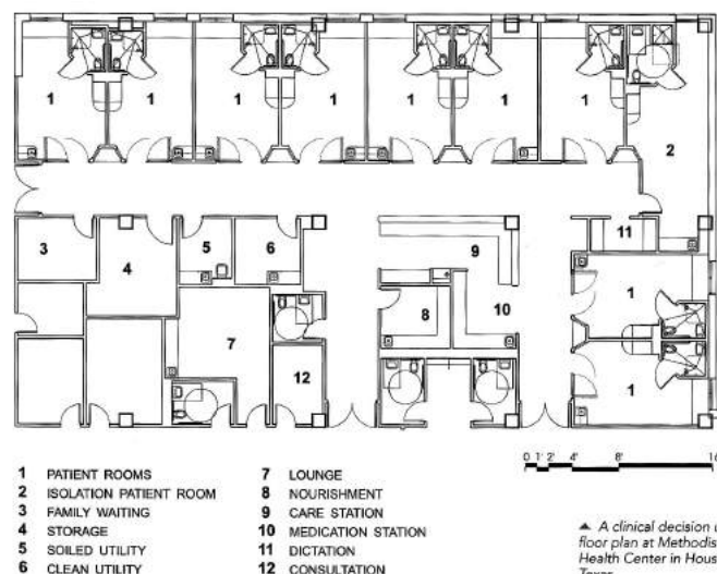
4.06. L shape nursing unit
