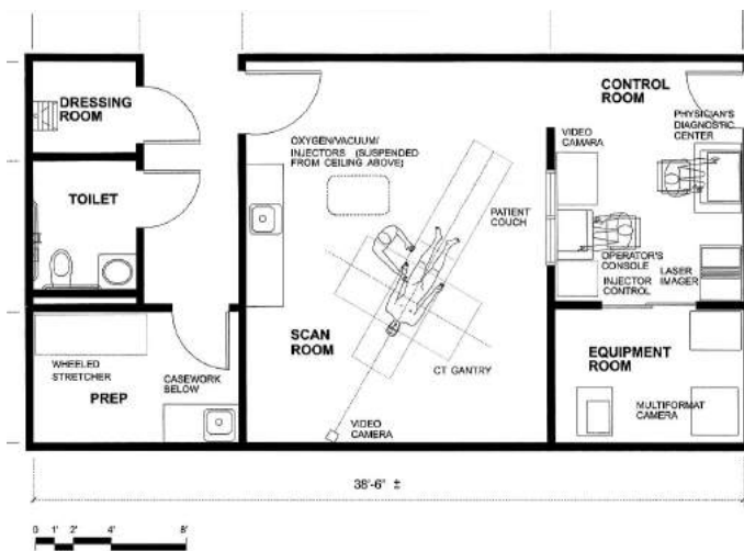
4.24. Computer Tomography unit, USA
