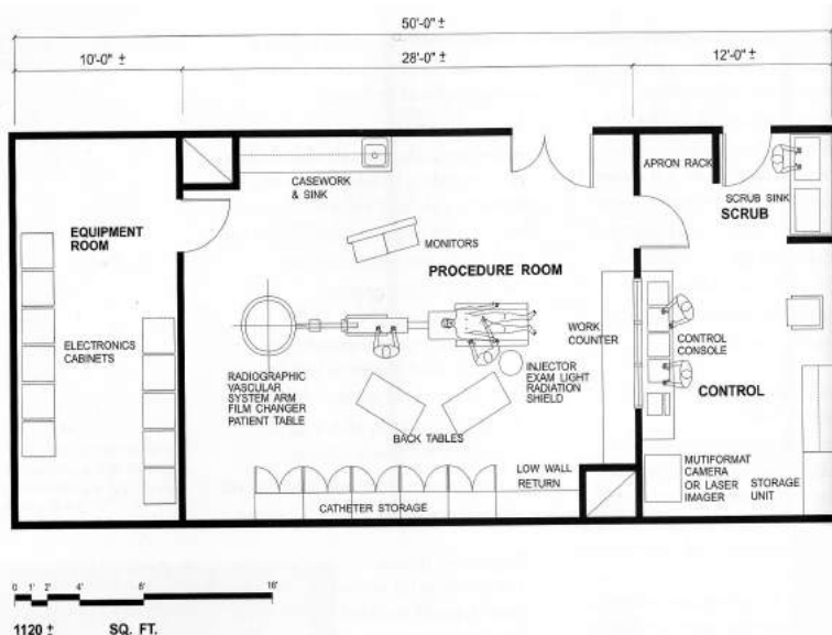
4.26. Typical special procedure angiography room at Medical Center East in Birmingham, Alabama, USA
