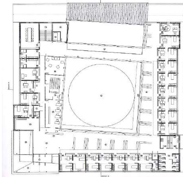
4.46. Polyclinic Centro de Salud, Ordes, A Coruna (2000.) Designer: Gabriel Santos ZAS
