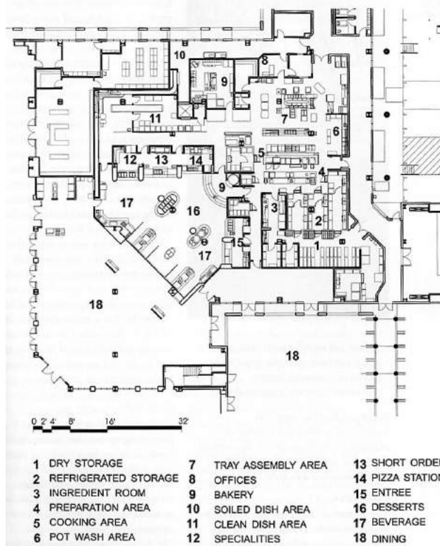
4.52. Dietary kitchen, Mercy Health Center, Laredo, Texas
